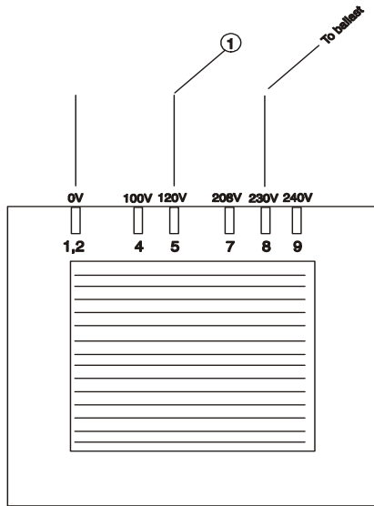
Transformer
